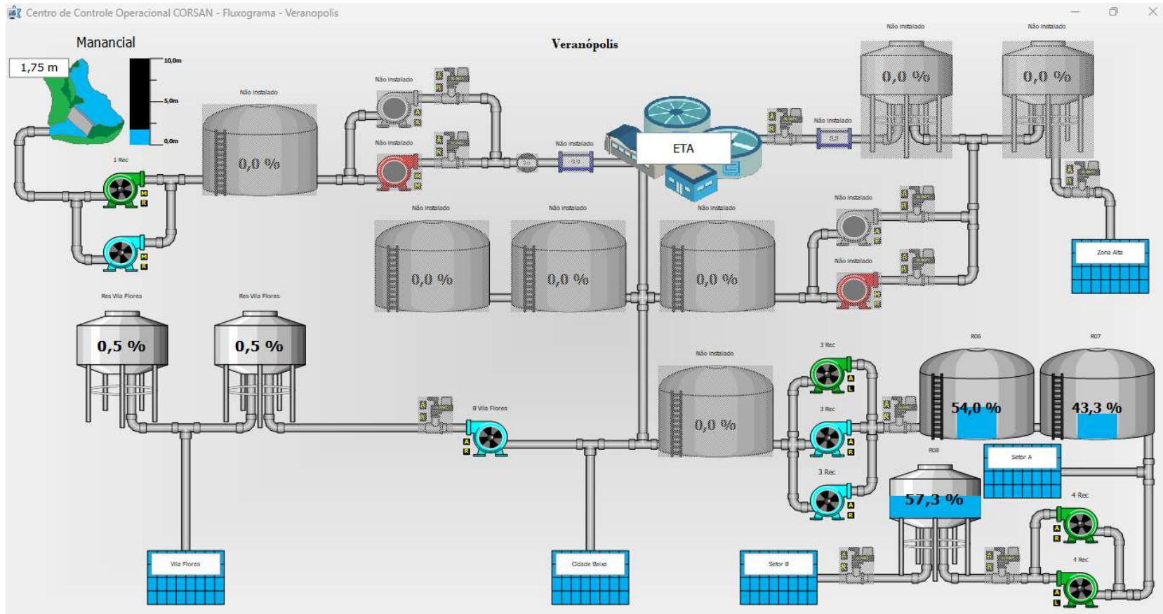
Figura 19 – Fluxograma do SAA (2/2).
